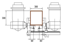
Profile machining centre SBZ 151 Edition 90
