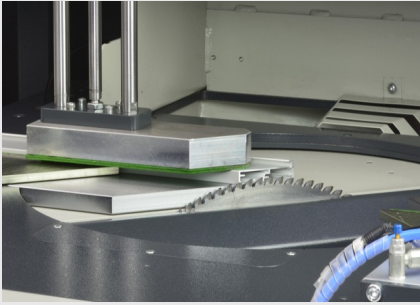
Cut-to-length centre SBZ 616/02
