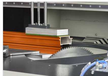
Cut-to-length centre SBZ 616/02
