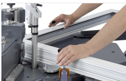
Corner crimper EP 124/20 2-hand operation
